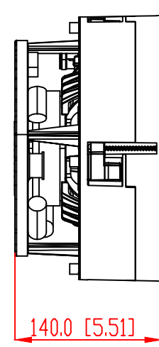
MOUNTING DEPTH
